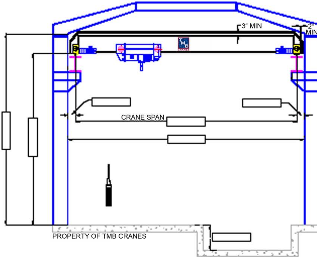
GENERAL CLEARANCE OUTLINE FOR TOP RUNNING CRANES
